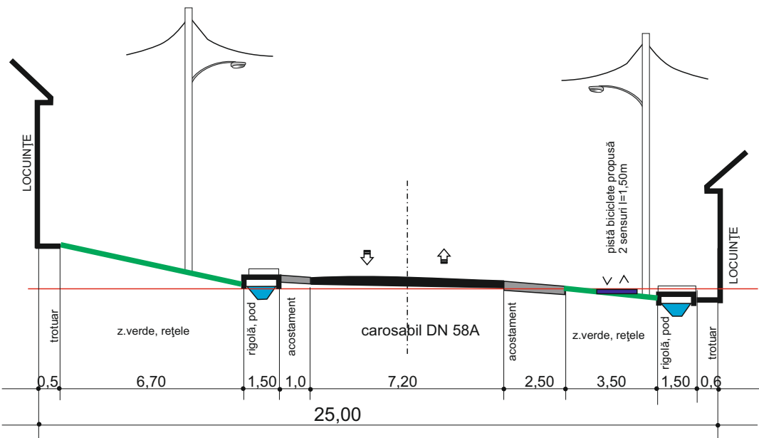
EZERIȘ profil caracteristic DN 58A sc. 1:250
